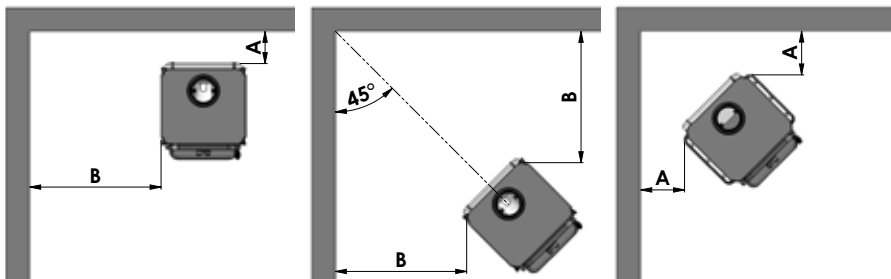
1412/1452 corner installation 1442 corner installation
